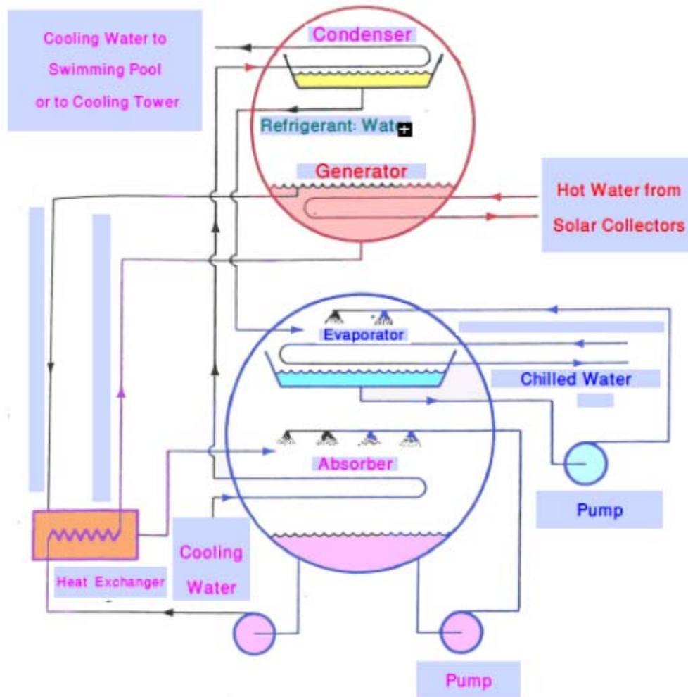
Absorbtion Chiller - Principle View
